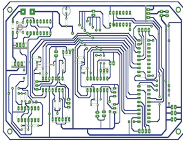
Fig 10.1 Main Board design using EAGLE
