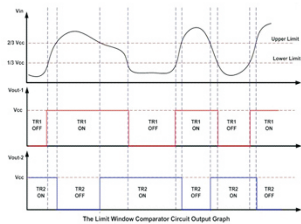
Fig 6.1.2 Output graph for the voltage sensing
