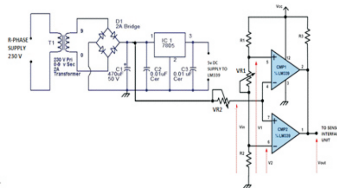
Fig 6.1 voltage comparator using lm339 limit window comparator
