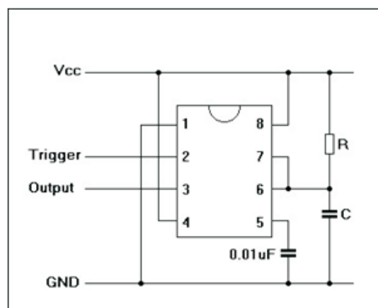
Fig 6.4 Monostable mode of Ne555
