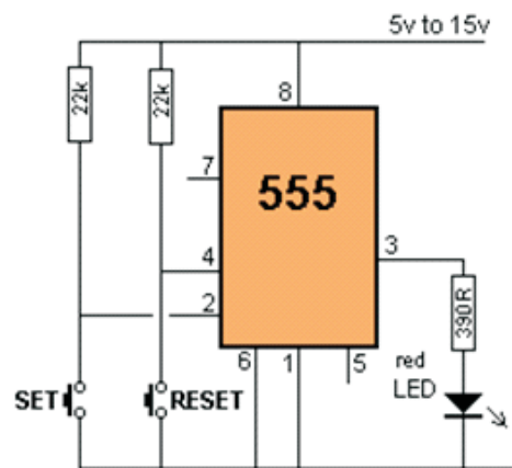
Fig 8.1 Latching using Ne555
