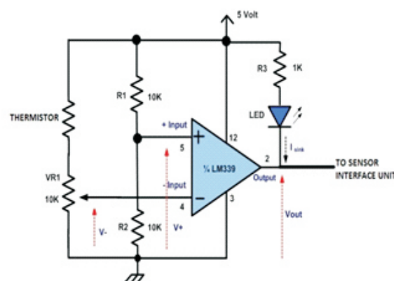
Fig 6.3 temperature sensing circuit
