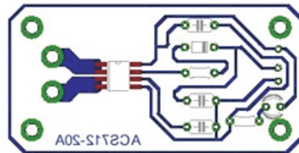
Fig 10.2 Current Sensor Board design using EAGLE
